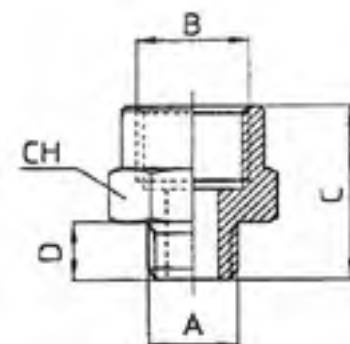
Conical Extension -BSPP
