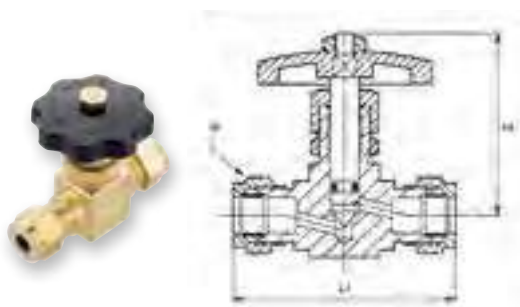
Straight Needle Valve Panel Mounting Tube- Tube-Imperial
