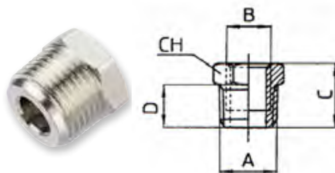
Reducing Bush -BSPT
