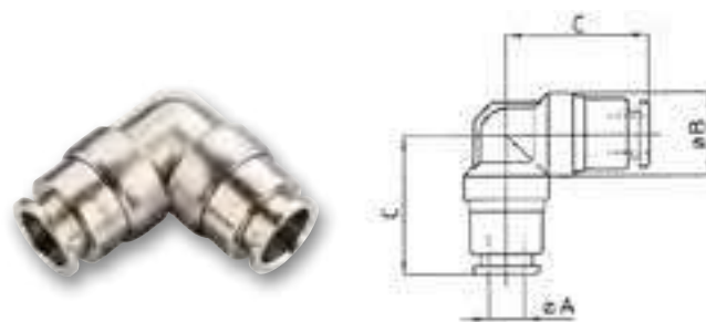
Equal Elbows
