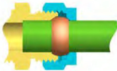
Spanner-Tight (After Compression)
