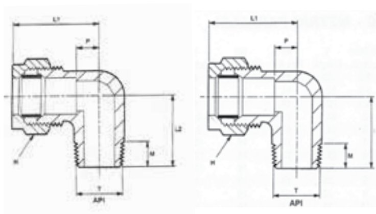
Male Stud Elbow API-Imperial
