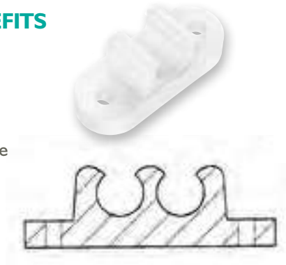
Nylorack Tube Clips-Imperial & Metric
