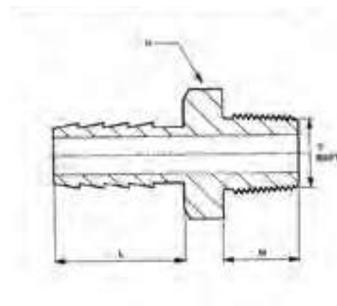
Hose Tail Adaptor BSPT Male-Imperial
