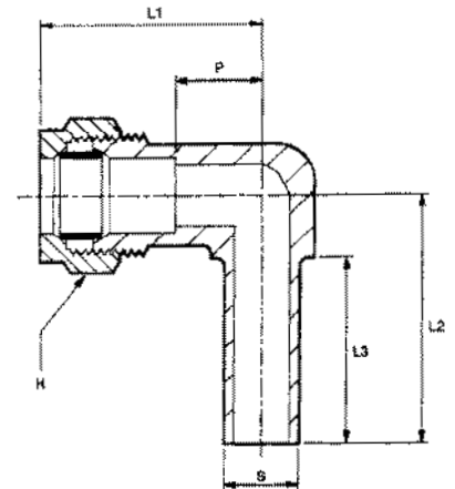
Standpipe Elbow-Imperial
