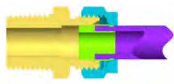
Spanner-Tight (After Compression)
