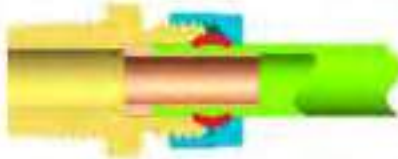
Spanner-Tight (After Compression)
