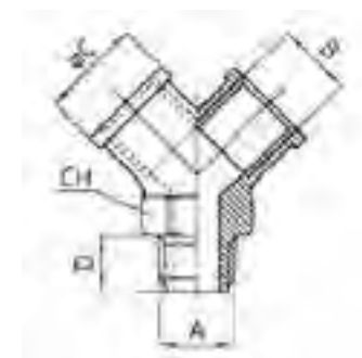
'Y' Connector Male BSPT -Female BSPP
