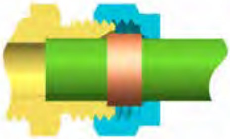
Finger-Tight (Before Compression)
