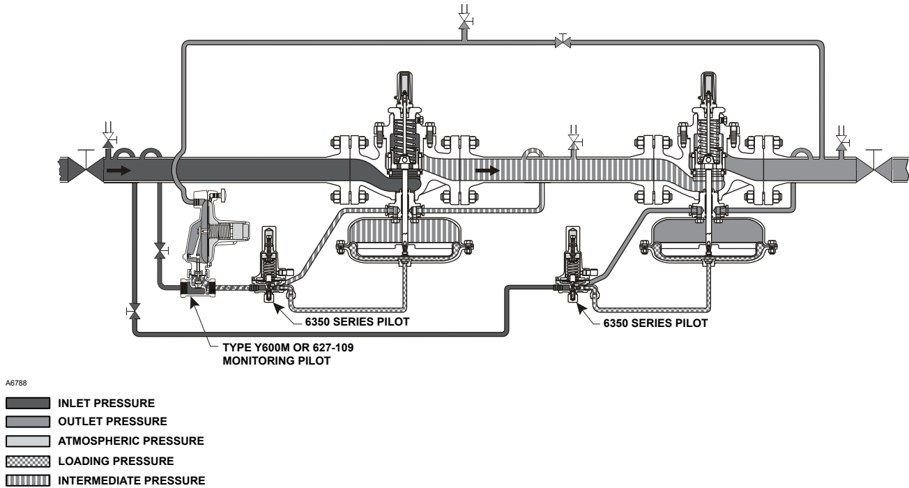
Figure 3. Working Monitor System
