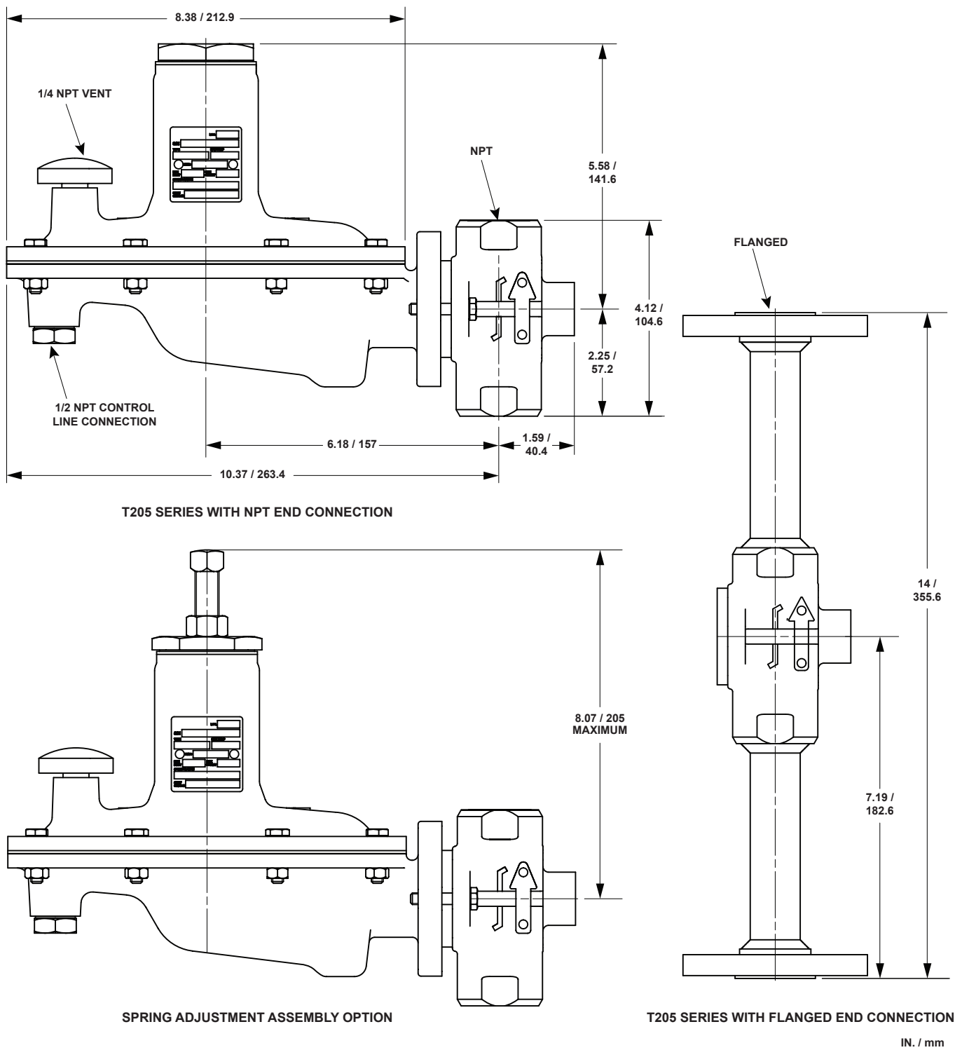
Figure 6. Dimensions
