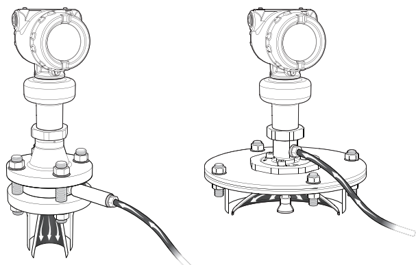
Figure 9. Air Purging
