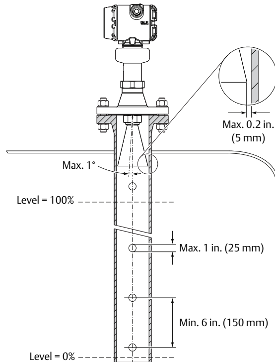
Figure 14. Still Pipe Requirements
