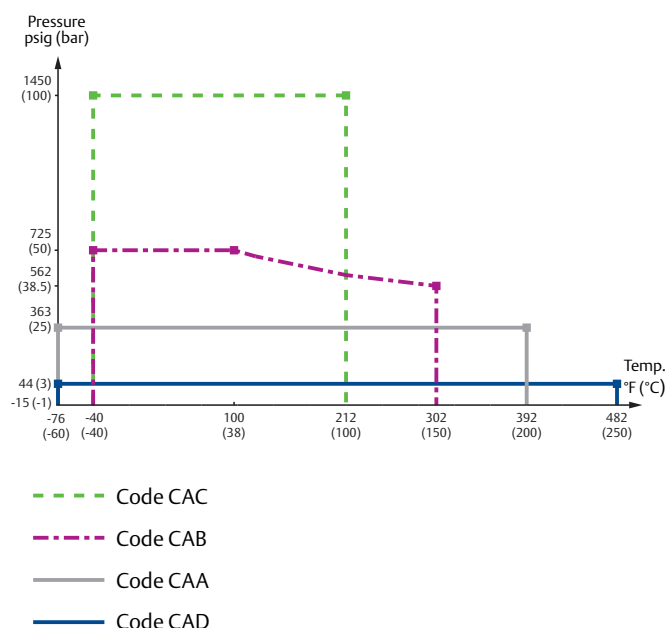
Figure 5. Cone Antenna (PTFE Seal) (1)
