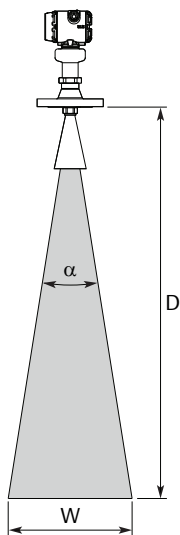
Figure 2. Beam Angle and Beam Width
