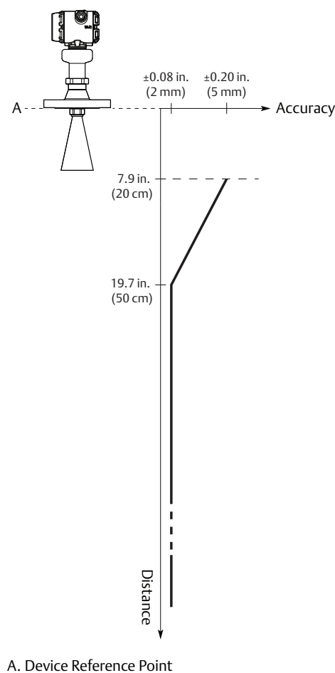
Figure 1. Accuracy Over Measuring Range
