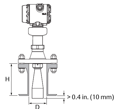
Figure 12. Mounting of the Cone Antenna
