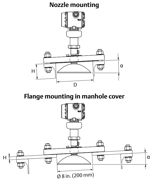
Figure 13. Mounting of the Parabolic Antenna
