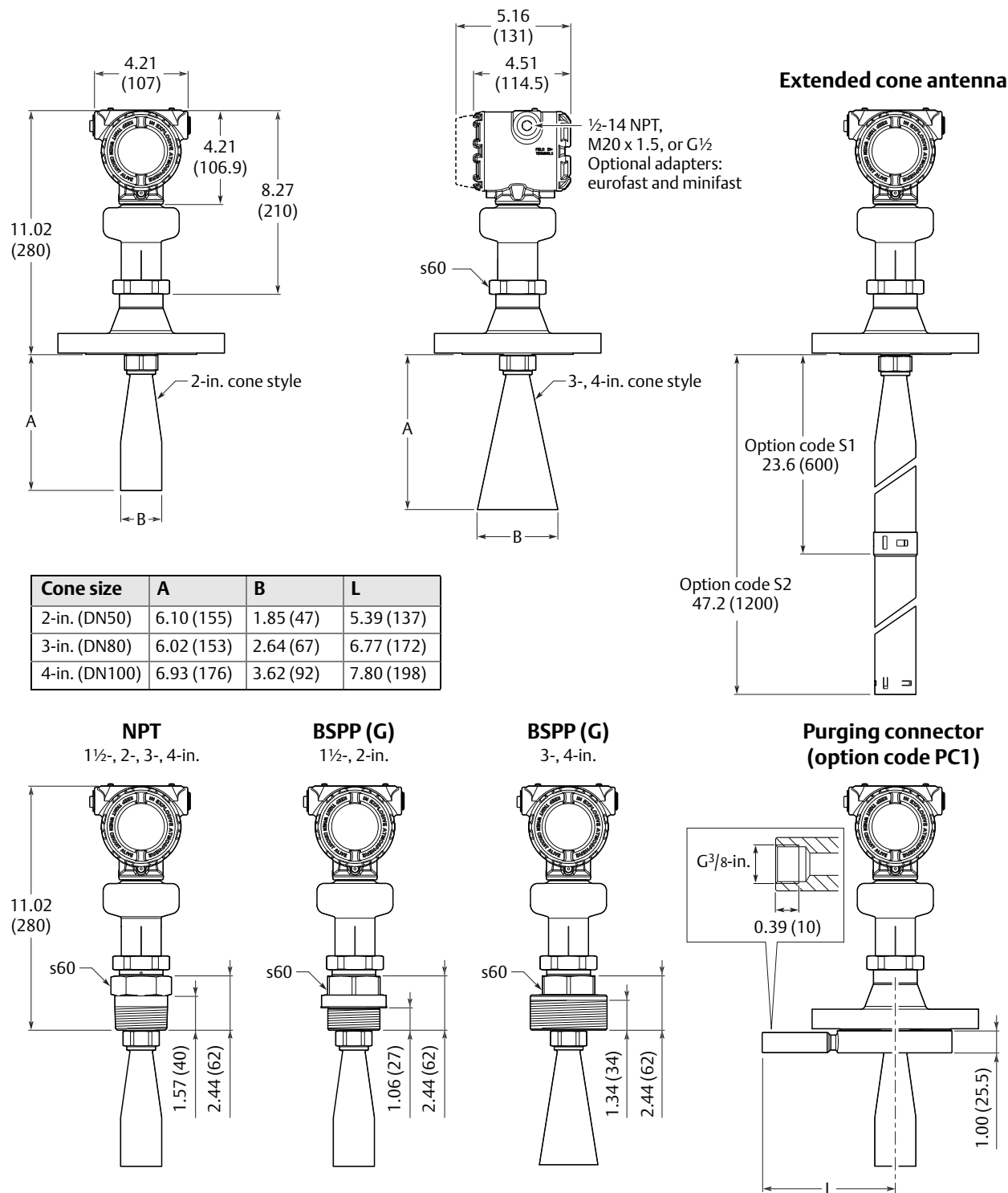
Figure 15. Cone Antenna
