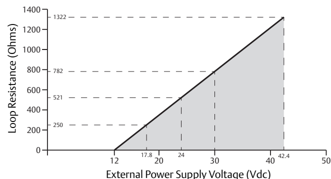
Figure 4. Load Limitations
