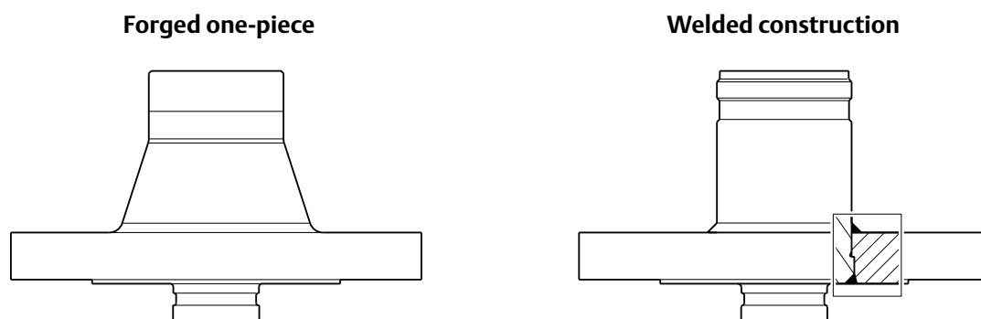
Figure 18. Cone Antenna Flange Connection
