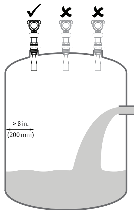
Figure 10. Recommended Mounting Position
