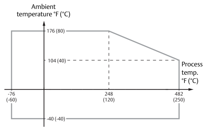
Figure 8. Ambient Temperature vs. Process Temperature
