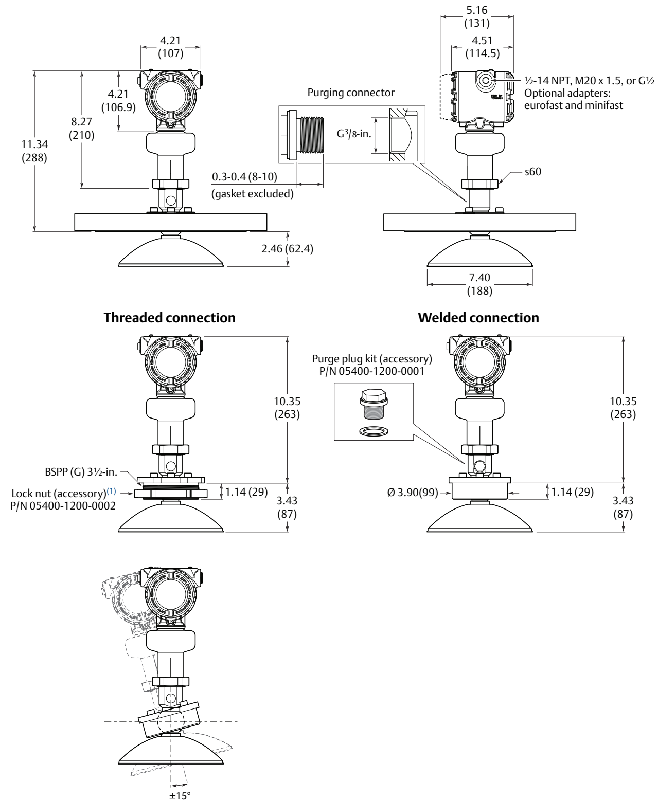
Figure 16. Parabolic Antenna
