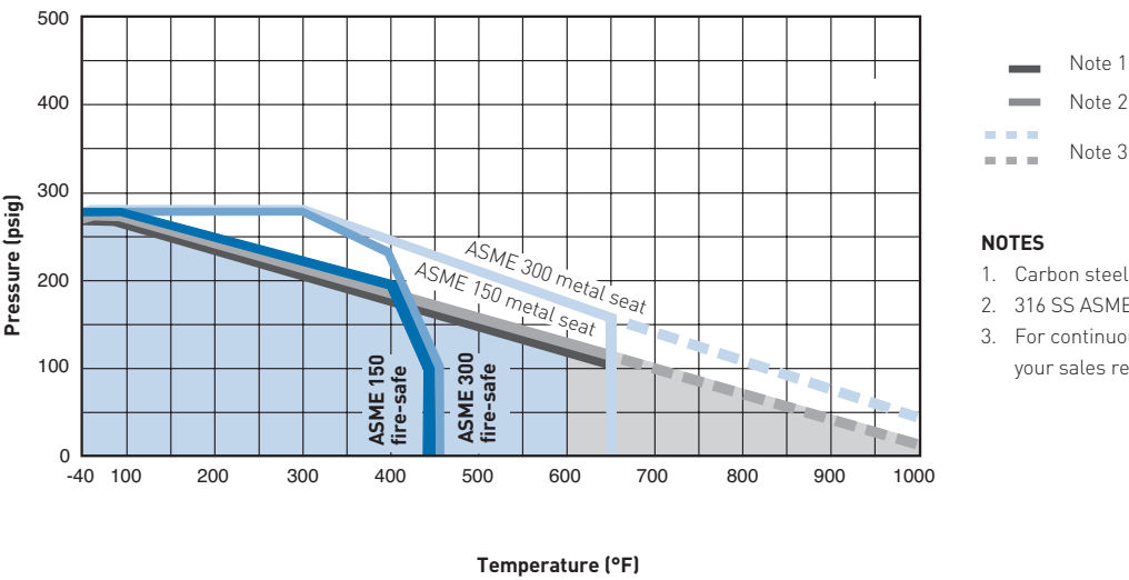
Fire-safe and metal seats
