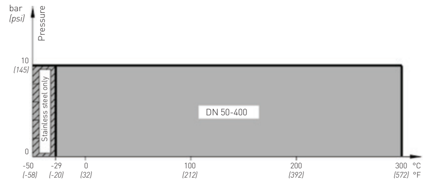
P/T DIAGRAM (HILOK PP SEAT)
