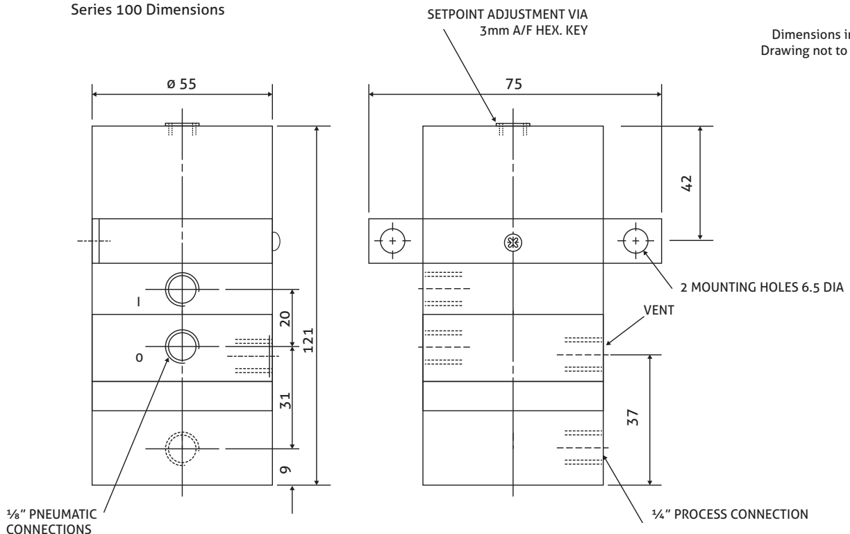
Series 100 Dimensions
