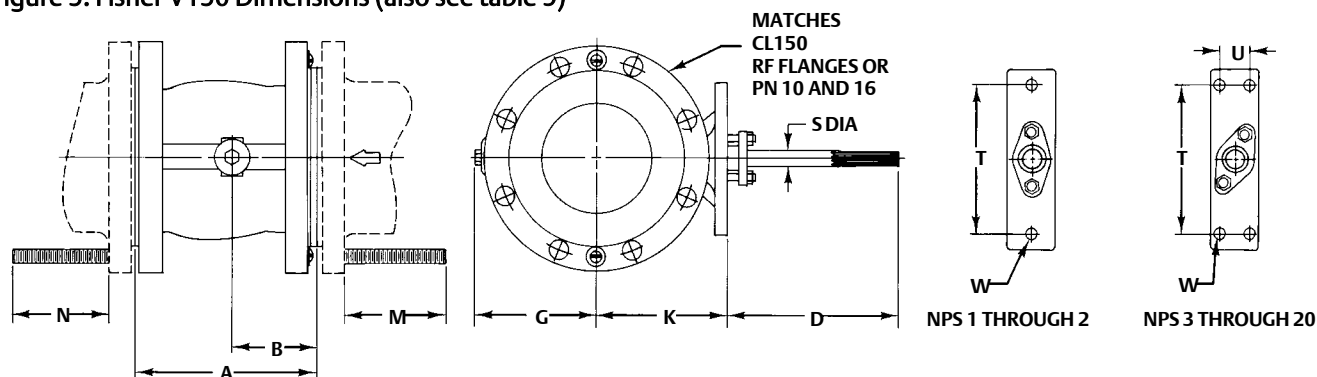
Figure 5. Fisher V150 Dimensions (also see table 9)
