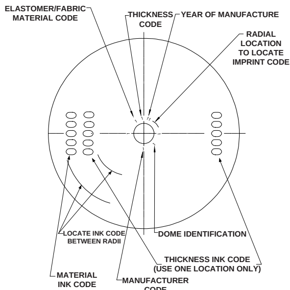
Figure 4. Diaphragm Markings
