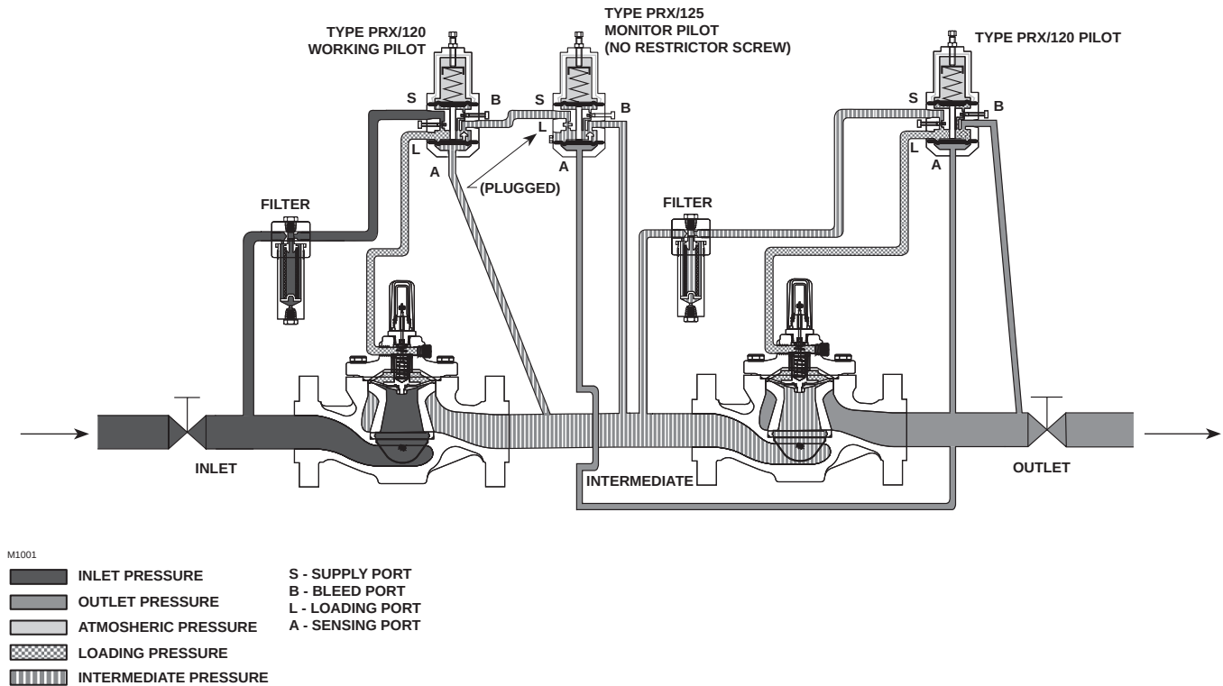
Figure 6. Type EZR-PRX-PRX Working Monitor Schematic
