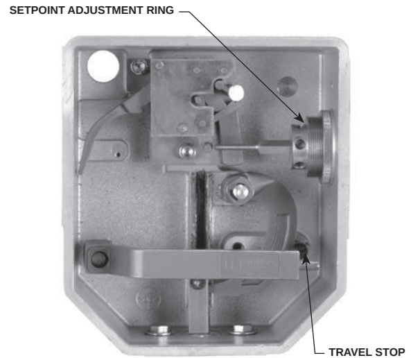
Figure 10. Slam-Shut Device in Closed Position
