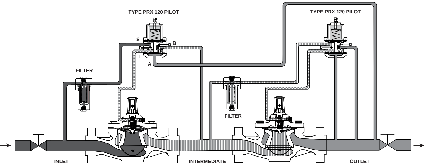
TYPE EZR-PRX WIDE-OPEN MONITOR WITH PILOT EXHAUST TO INTERMEDIATE PRESSURE WITH PILOT EXHAUST TO INTERMEDIATE PRESSURE
