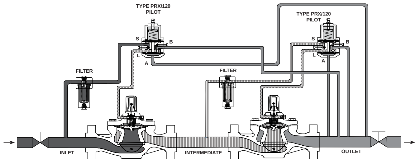
TYPE EZR-PRX WIDE-OPEN MONITOR
