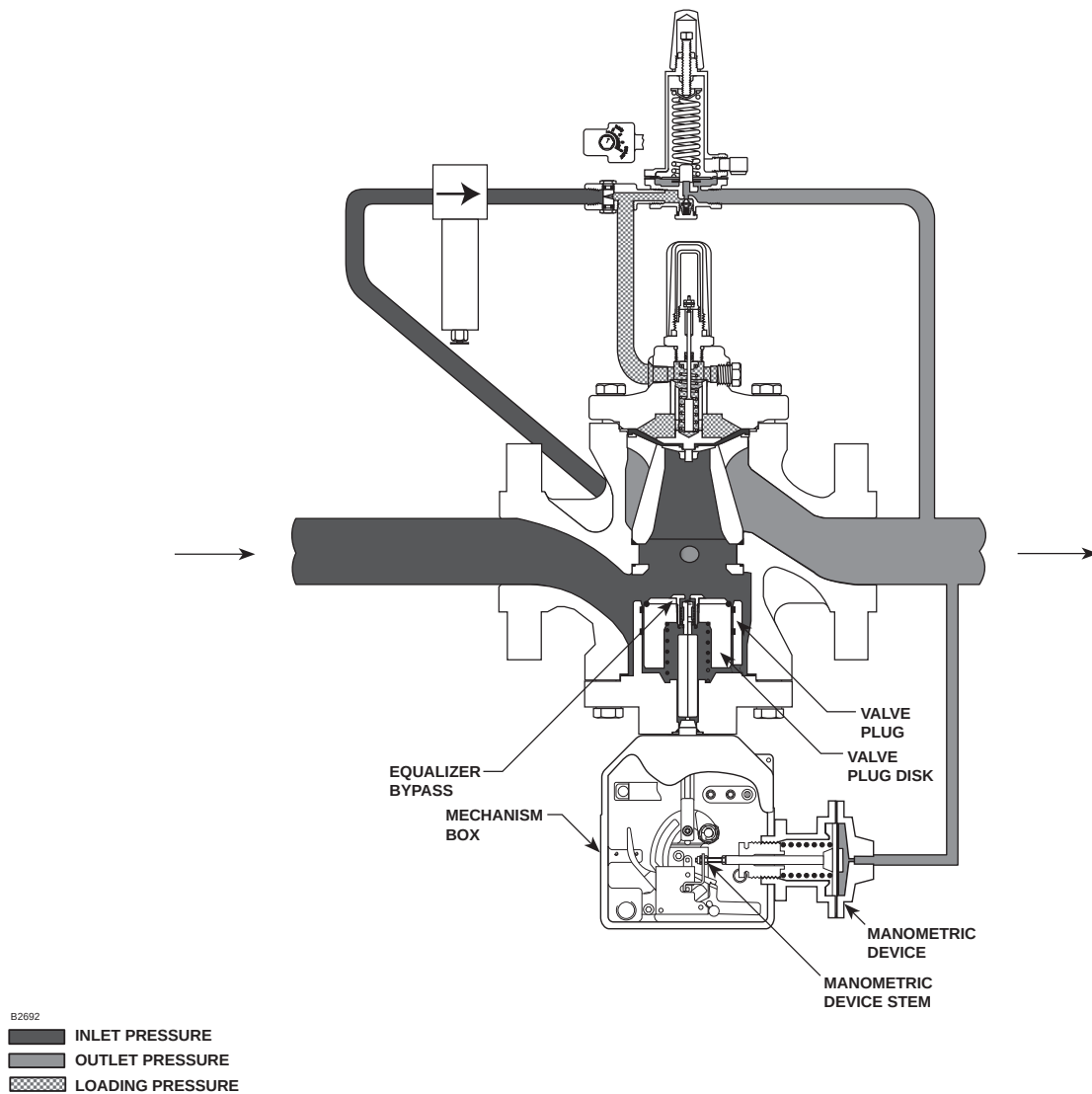
Figure 7. Type EZROX with Slam-shut Device Operational Schematic
