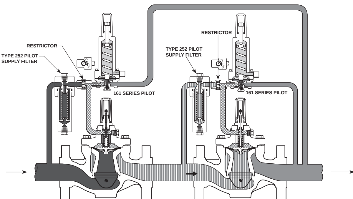
TYPE EZR-161 WIDE-OPEN MONITOR
