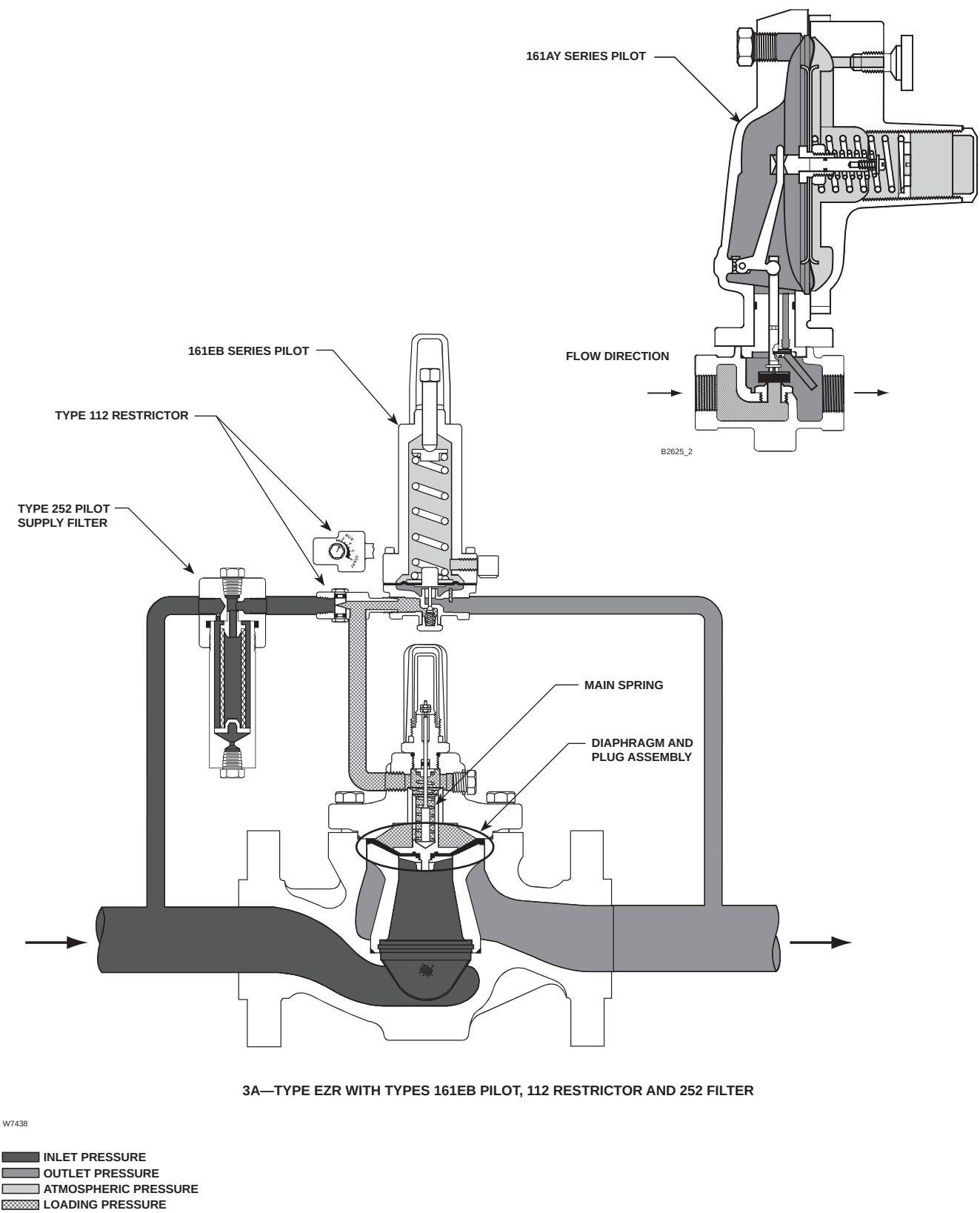
Figure 3. Type EZR Operational Schematic
