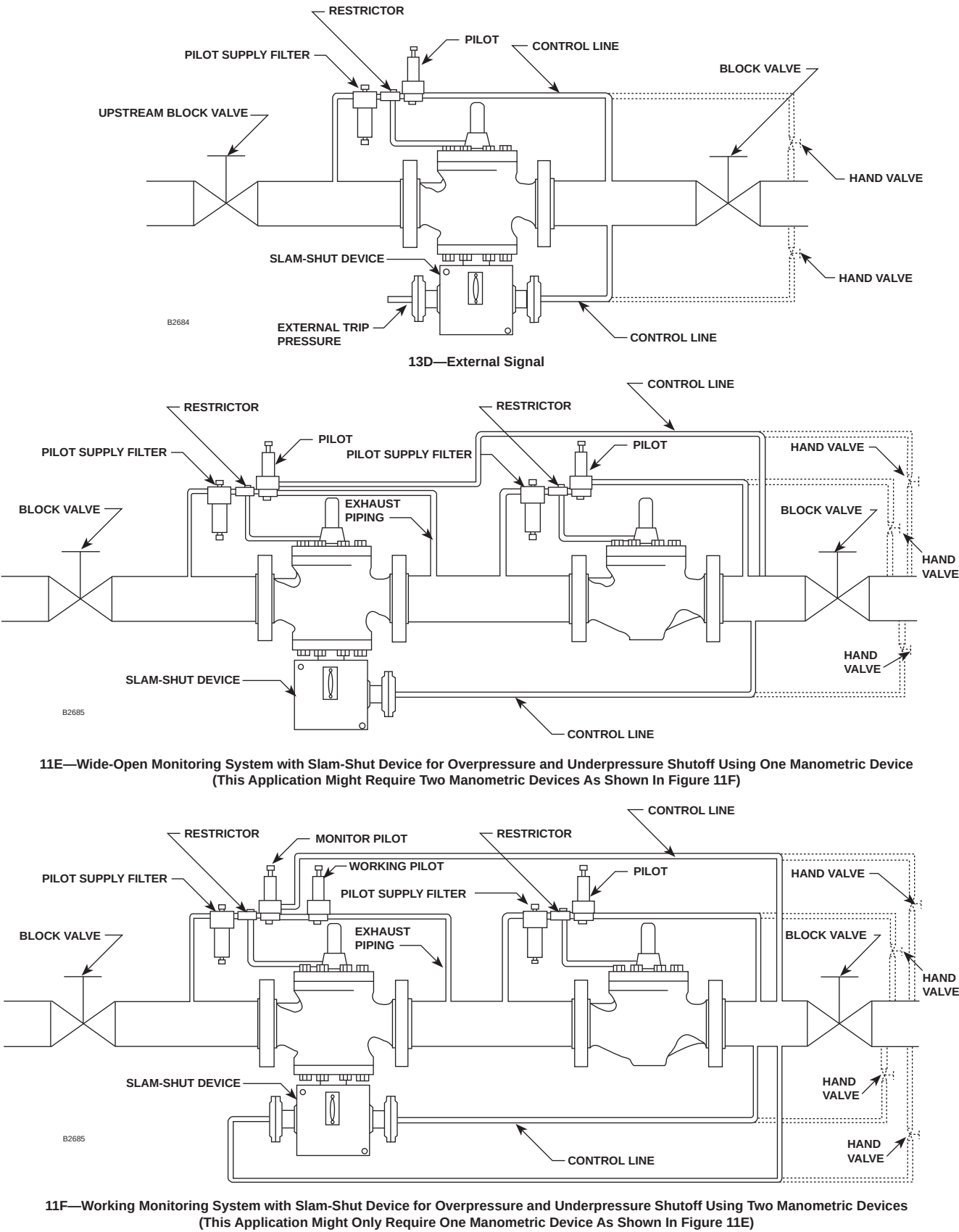
Figure 11. Type EZROX with Integral Slam-Shut Device Installation Schematics (continued)
