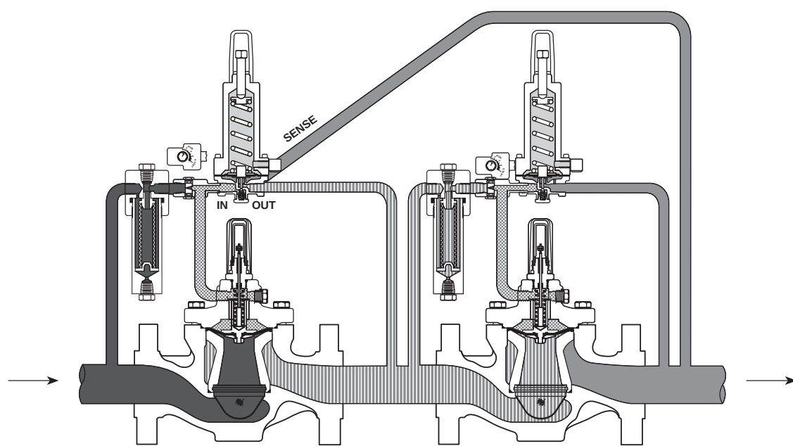
TYPE EZR-161 WIDE-OPEN MONITOR WITH PILOT EXHAUST TO INTERMEDIATE PRESSURE
