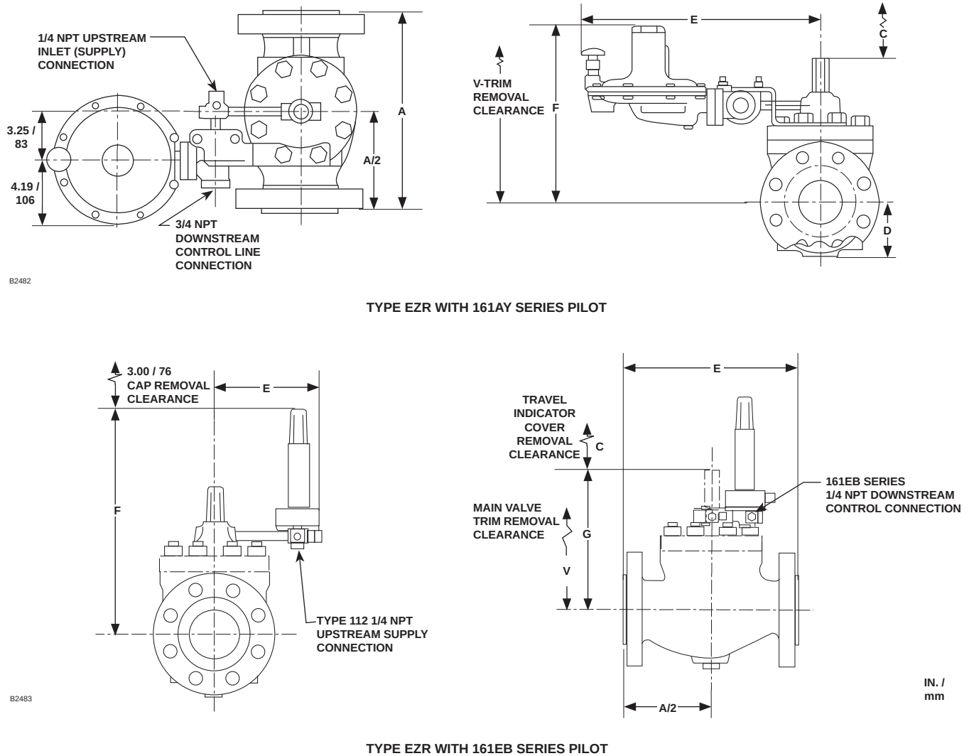
Figure 12. Typical EZR Dimensions
