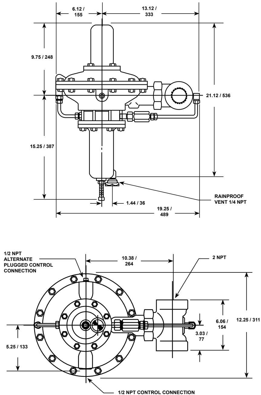
Figure 15. Type 99 (NPT) with Type 61H Pilot Dimensions
