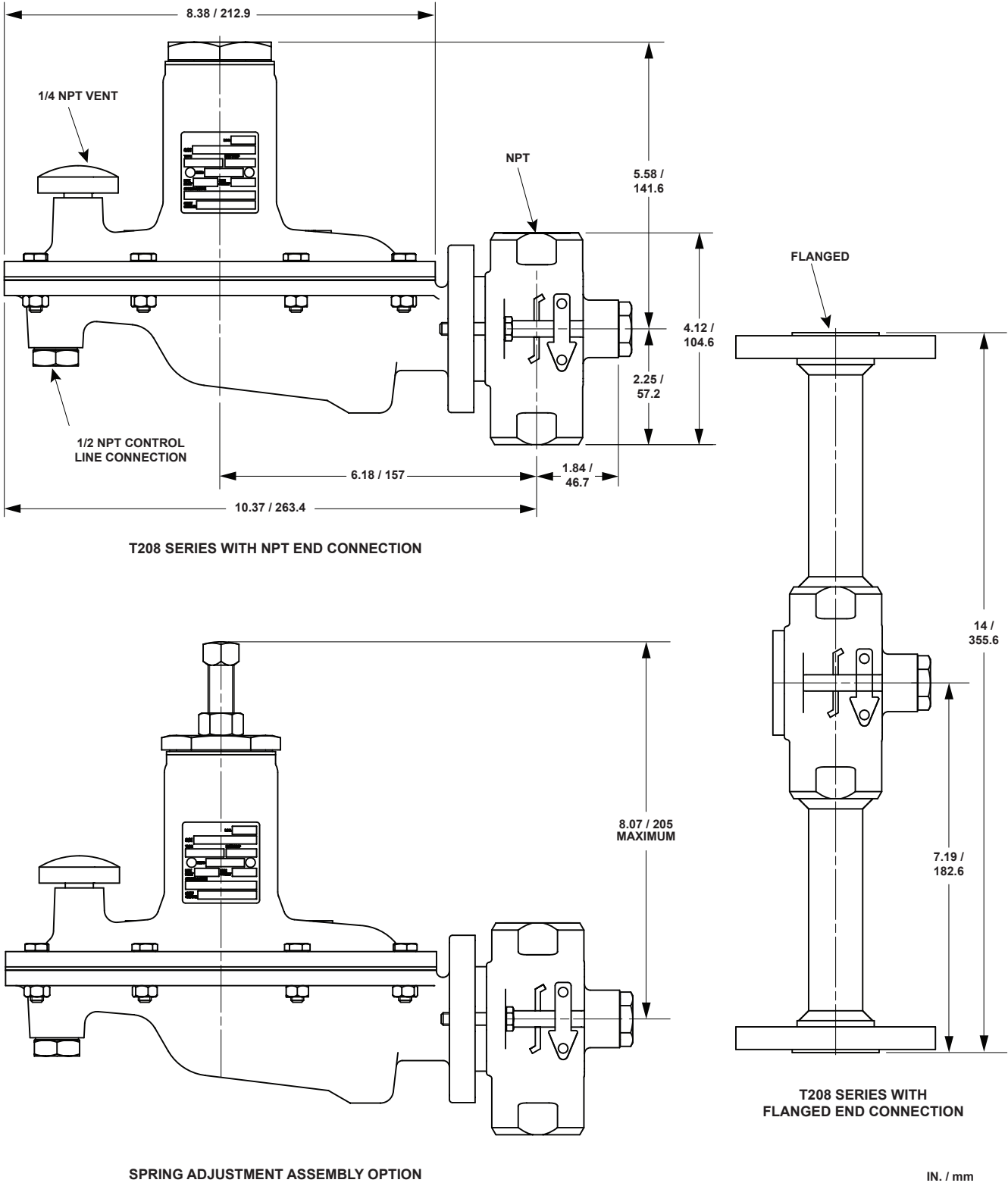
Figure 5. Dimensions
