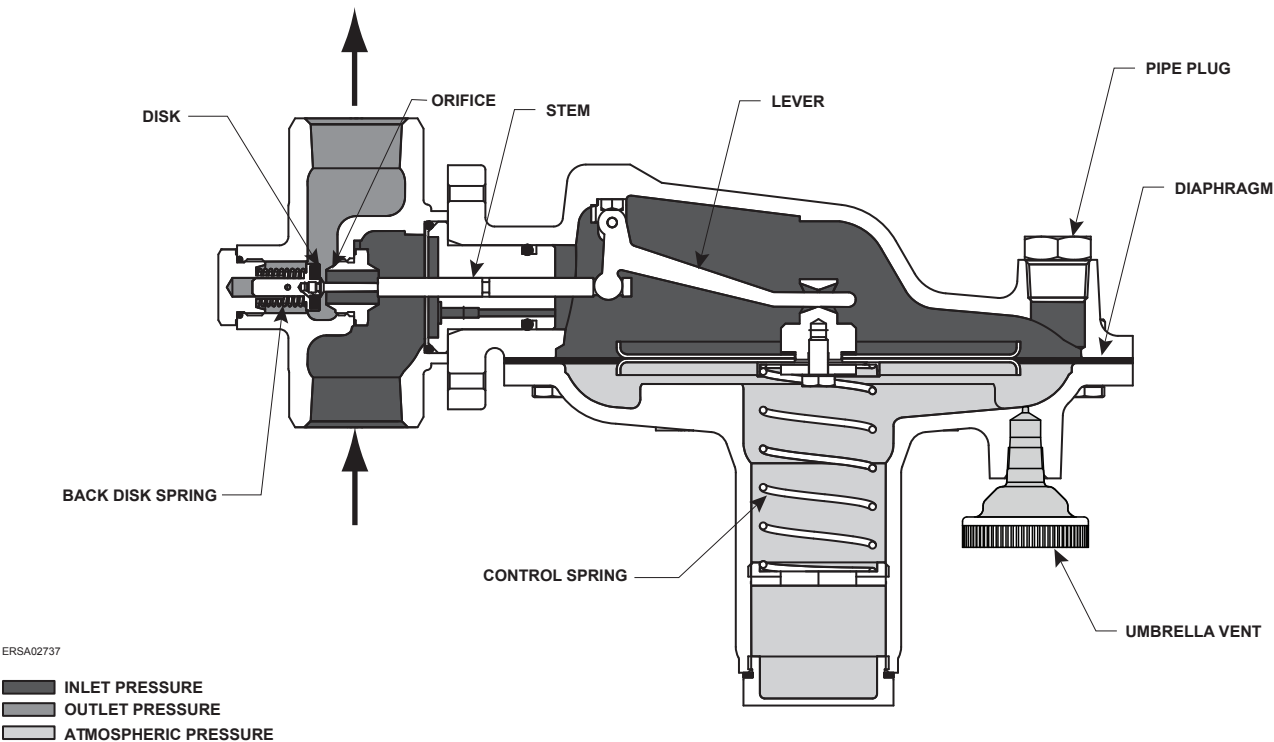
Figure 2. Type T208 with Internal Pressure Registration Operational Schematics
