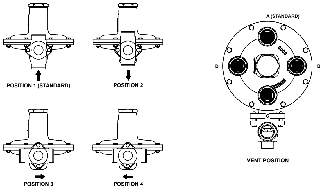
Figure 4. Body and Vent Orientation
