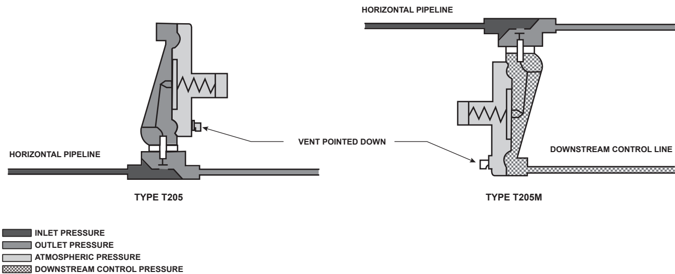
Figure 4. T205 Series Actuator Casing Drainage Schematic
