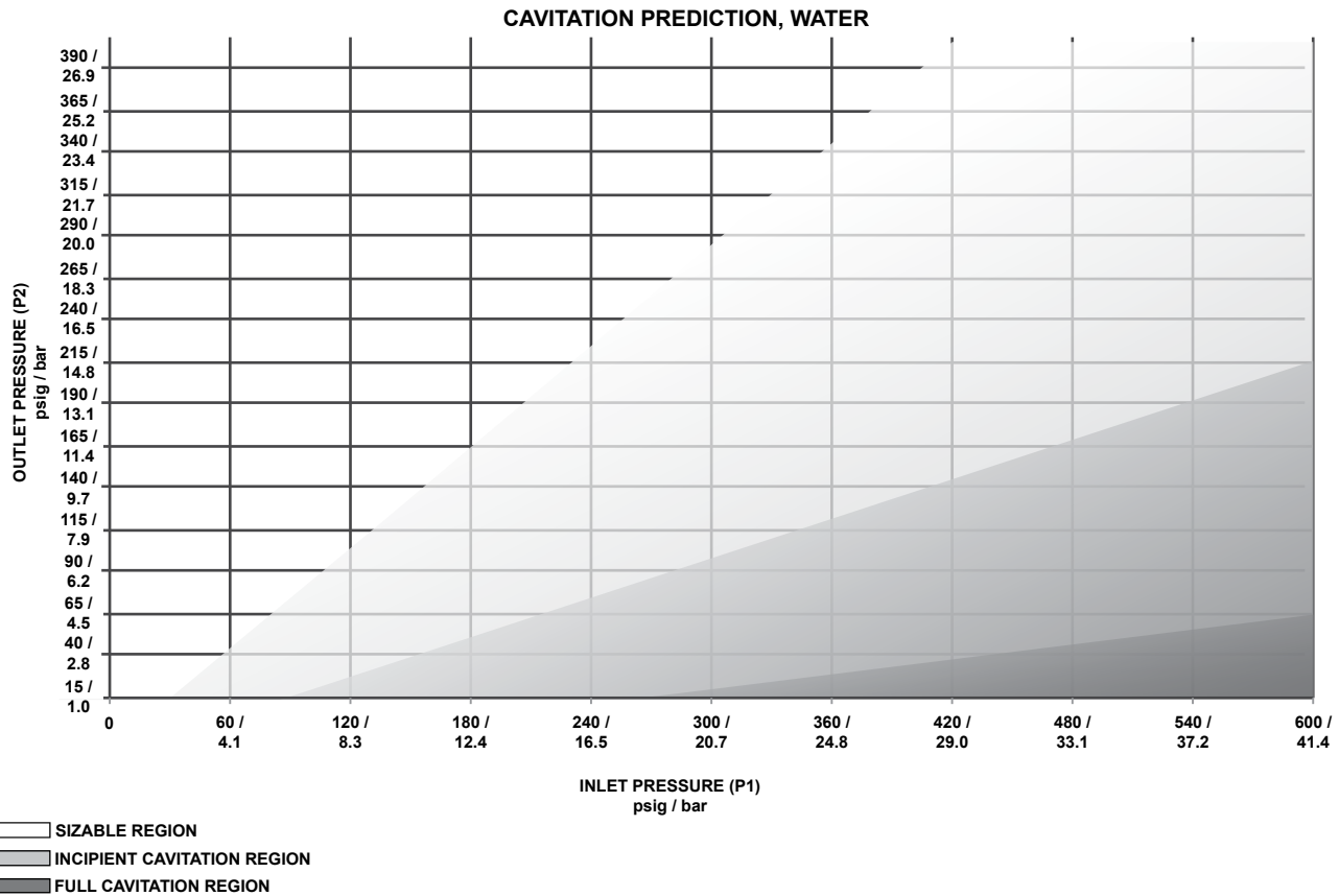
Figure 4. Cavitation Sizing for Water
