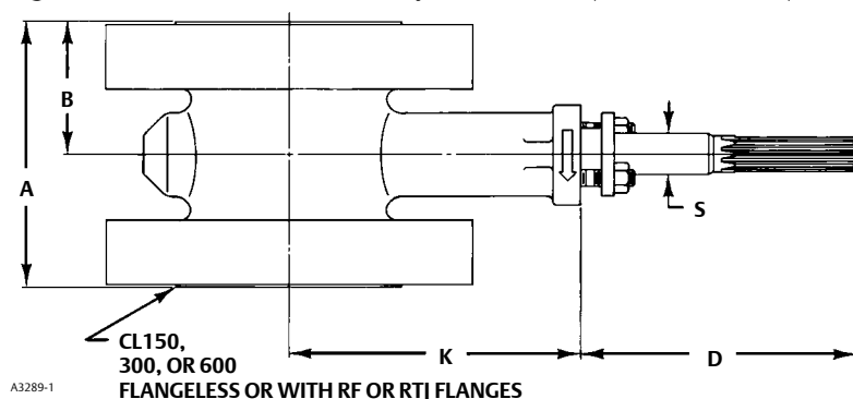
Figure 4. Fisher CV500 Valve Body Dimensions (also see table 6)
