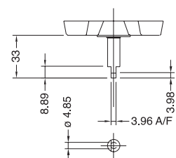
NAMUR shaft details
